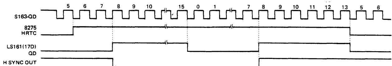
Fig 7 - 26 Horizontal Sync. Timing
