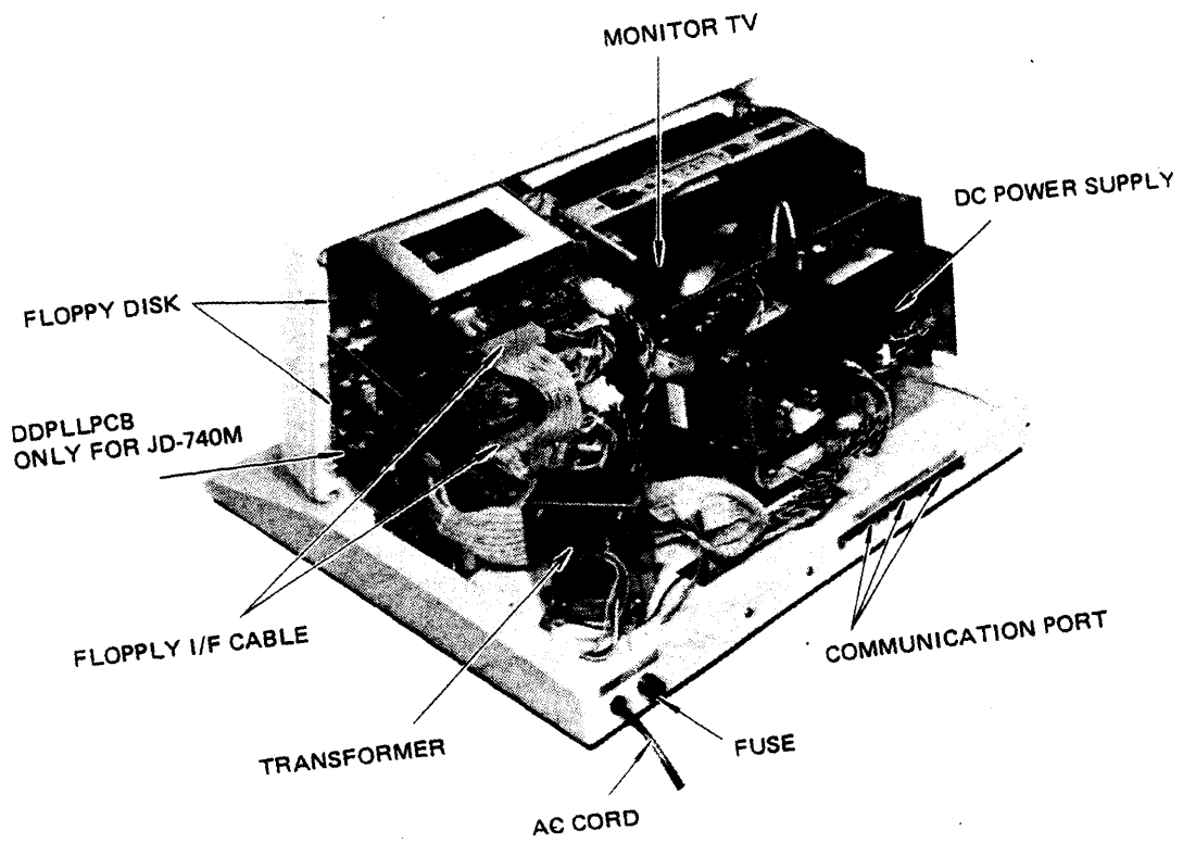
Fig. 2 - 3 JD-700M SERIES INTERNAL LAYOUT
