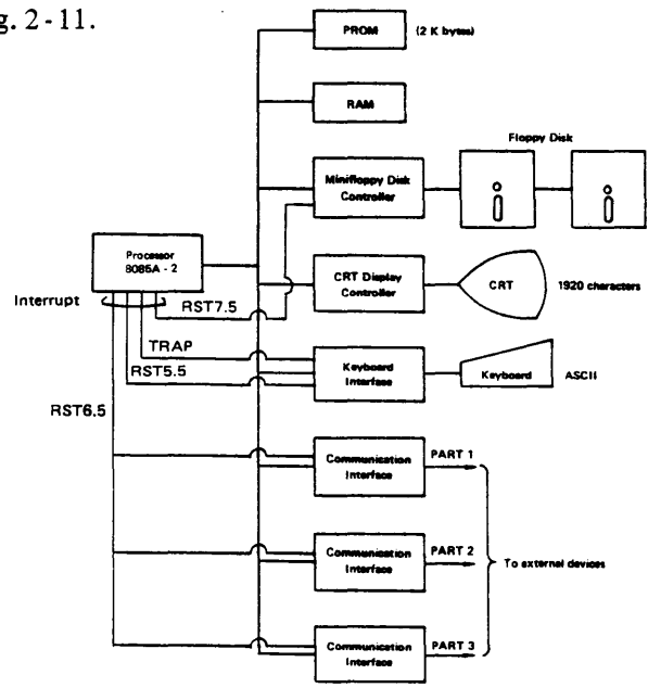
Fig. 2 - 14 FUNCTION BLOCK DIAGRAM
