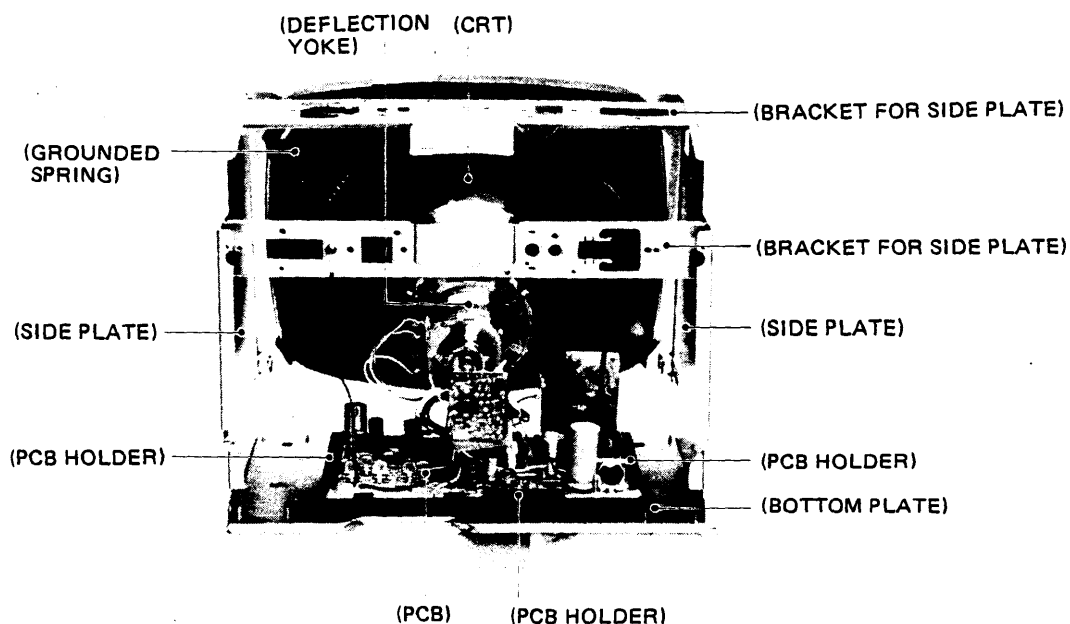
Fig. 5 - 1 LAYOUT (1/2)
