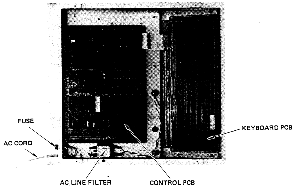
Fig. 2 - 6 JD-700M/740M/800M/840M INTERNAL LAYOUT (FROM BOTTOM)
