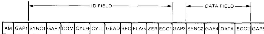
FIGURE 4-6 SECTOR FORMAT
