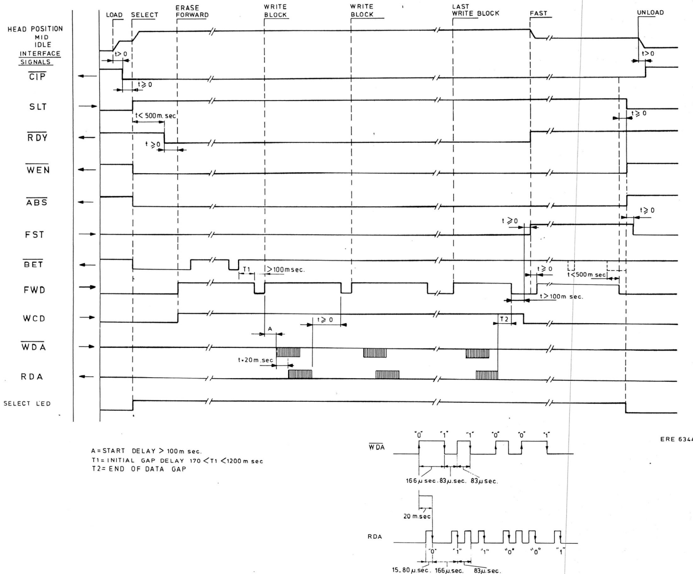
TIMING DIAGRAM DCR 4B
