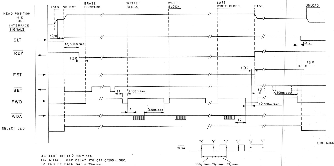
TIMING DIAGRAM DCR 4A
