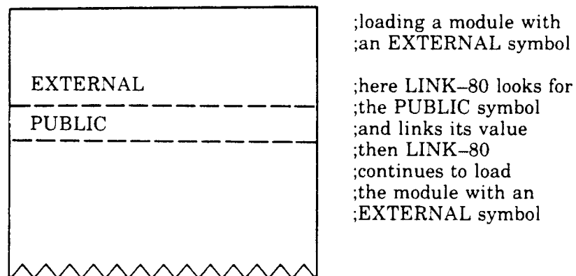
Figure 1.2: PUBLIC symbol linked into module at EXTERNAL
